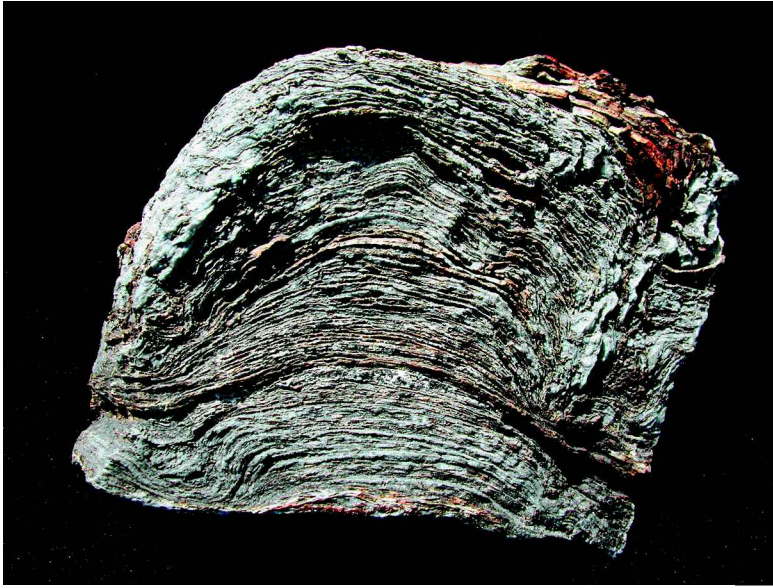
GOAL 7. Stromatolite, Transvaal Dolomite, 2.5 billion years old, Republic of South Africa. Courtesy of D. Des Marais, Ames Research Center, NASA.
