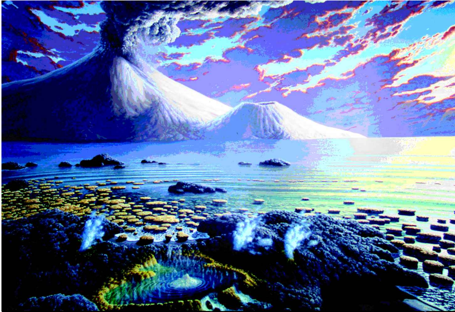
GOAL 4. Archean world, 3.5 billion years ago. Courtesy of the Smithsonian Institution, Peter Sawyer, artist.
