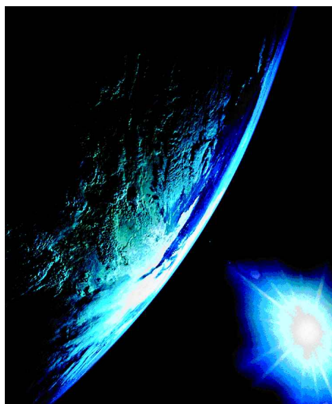
GOAL 6. The environments of Earth and space. Courtesy of C. Triano, Boomerang Design.
