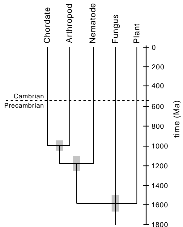
Figure 3. Divergence times and relationships of metazoan phyla and of plants, animals and fungi. Shaded bars denote 1 s.e.m.
