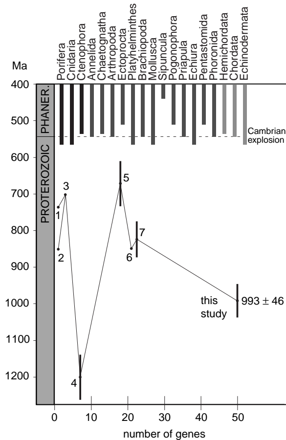
Figure 1. Time of divergence between animal phyla (protostome–deuterostome) as measured by different studies and here (numbers correspond to the following studies: 1, Brown et al. 1972; 2, Runnegar 1982; 3, Runnegar 1986; 4, Wray et al. 1996; 5, Ayala et al. 1998; 6, Feng et al. 1997; and 7, Gu 1998). Vertical bars at top indicate fossil record of living phyla (black, basal animal phyla; medium grey, protostomes; light grey, deuterostomes). Only those phyla known from the early Phanerozoic are shown. Standard errors are shown only for those studies where that statistic was reported.
