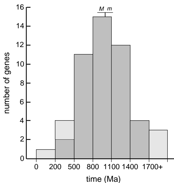
Figure 2. Distribution of divergence times between chordates and arthropods. Mean, M ; median, m . Dark shading denotes time estimates used in analysis; light shading denotes outliers.
